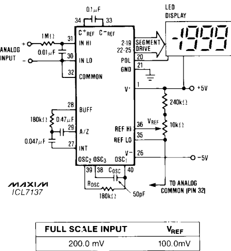
Figure 2. Maxim ICL7137 Typical Operating Circuit Clock Frequency 48kHz (3 reading/sec)
