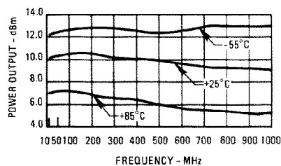
Power Output*
