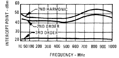
Intercept Point
