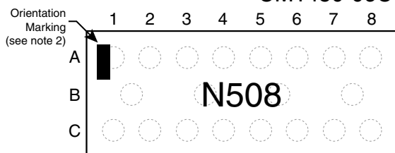
CM1450-06CS/CP 15-Bump CSP Package
