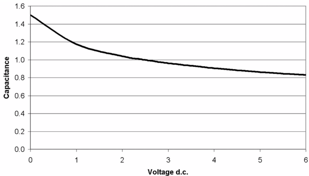
Figure 2. Filter Capacitance vs. Input Voltage over Temperature (normalized to capacitance at 2.5VDC and 25^\circ\text{C} )
