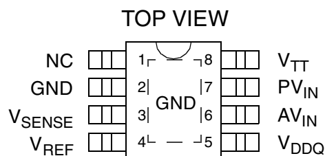
8-lead PSOP
