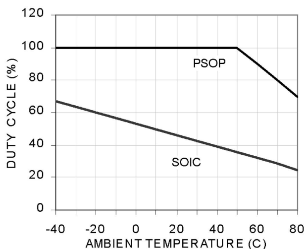
Figure 10. Duty Cycle vs. Ambient Temperature ( I_{LOAD}=2.0\text{A} )
