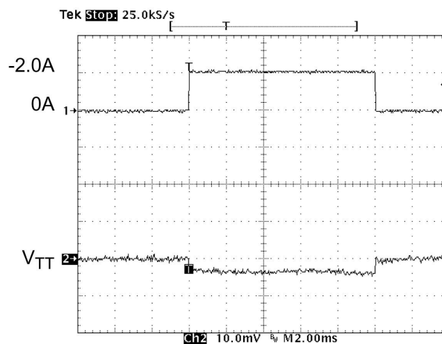
Figure 9. Line Transient (0A to 2.0A Source)
