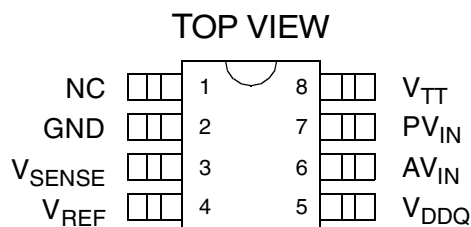
8-lead SOIC
