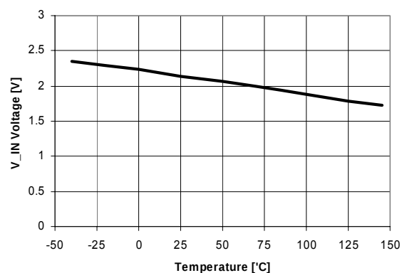
Undervoltage lockout
