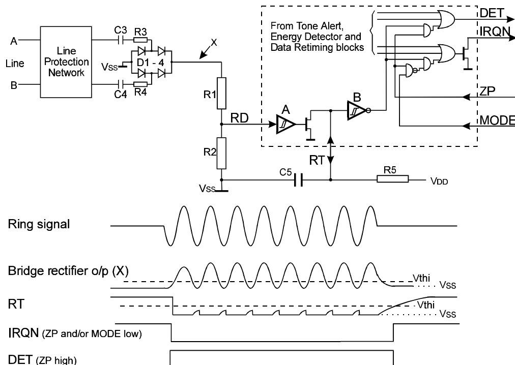
Figure 7 : Ring or Line Polarity Reversal operation
