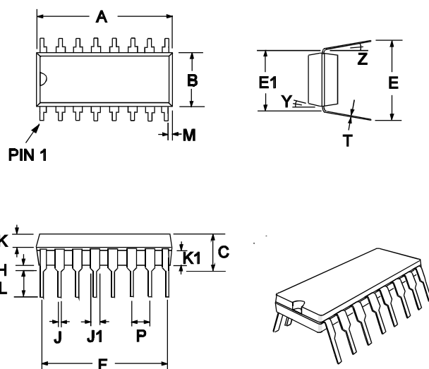
Figure 13 : 16-pin DIL (P3) Mechanical Outline: Order as part no. CMX602AP3
