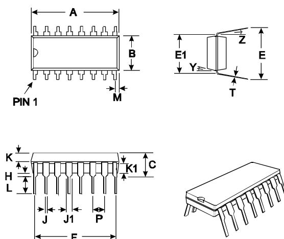
Figure 9 16-pin SOIC (D4) Mechanical Outline: Order as part no. CMX605D4
