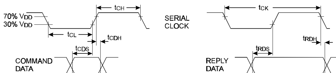
Figure 8 'C-BUS' Timing
