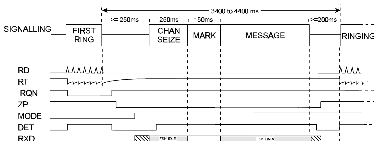
Figure 9b : Bellcore On-hook System Signals
