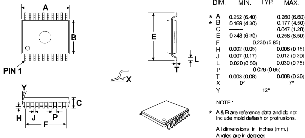
Figure 14 : 20-pin TSSOP (E3) Mechanical Outline: Order as part no. CMX612E3
