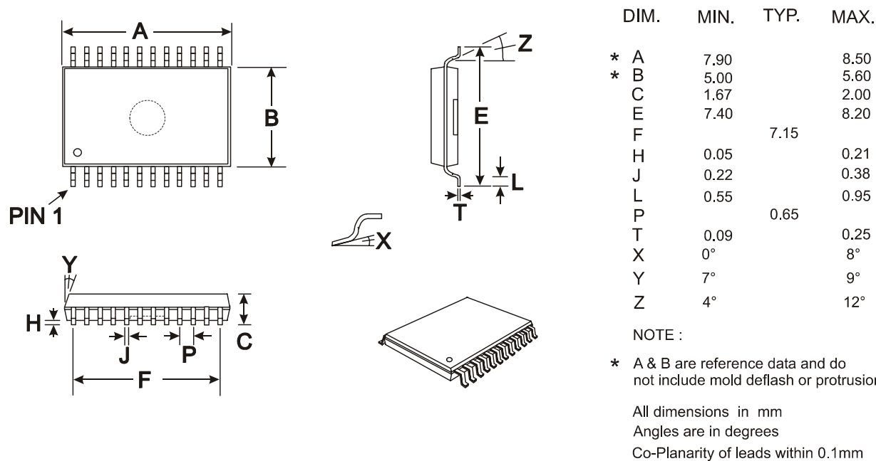
Figure 12b 24-pin SSOP (D5) Mechanical Outline: Order as part no. CMX624D5
