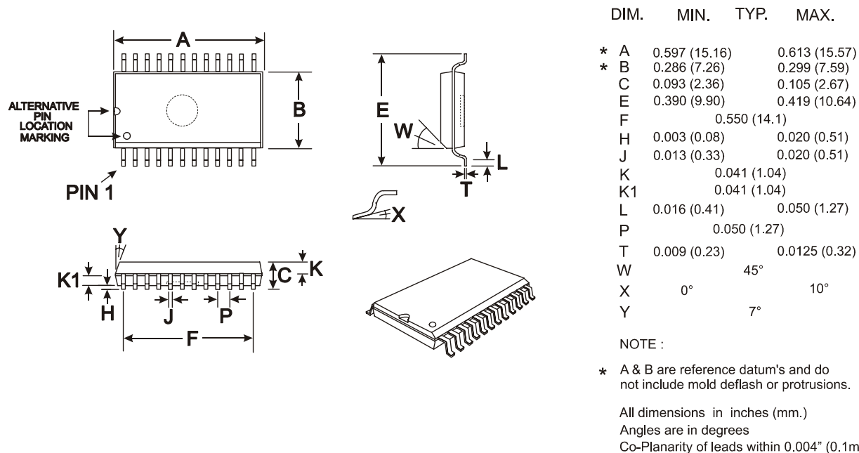
Figure 12a 24-pin SOIC (D2) Mechanical Outline: Order as part no. CMX624D2
