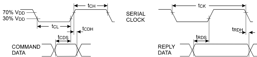
Figure 10 'C-BUS' Timing
