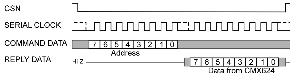
Figure 7 'C-BUS' Transactions
