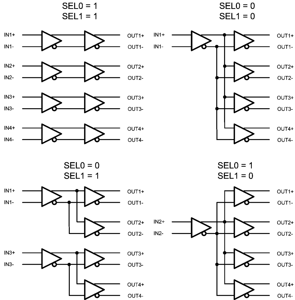
FIGURE 1. DS90CP04 Configuration Select Decode
