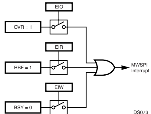
Figure 37. MWSPI Interrupts
