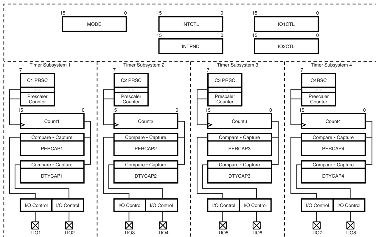
Figure 50. Versatile Timer Unit Block Diagram
