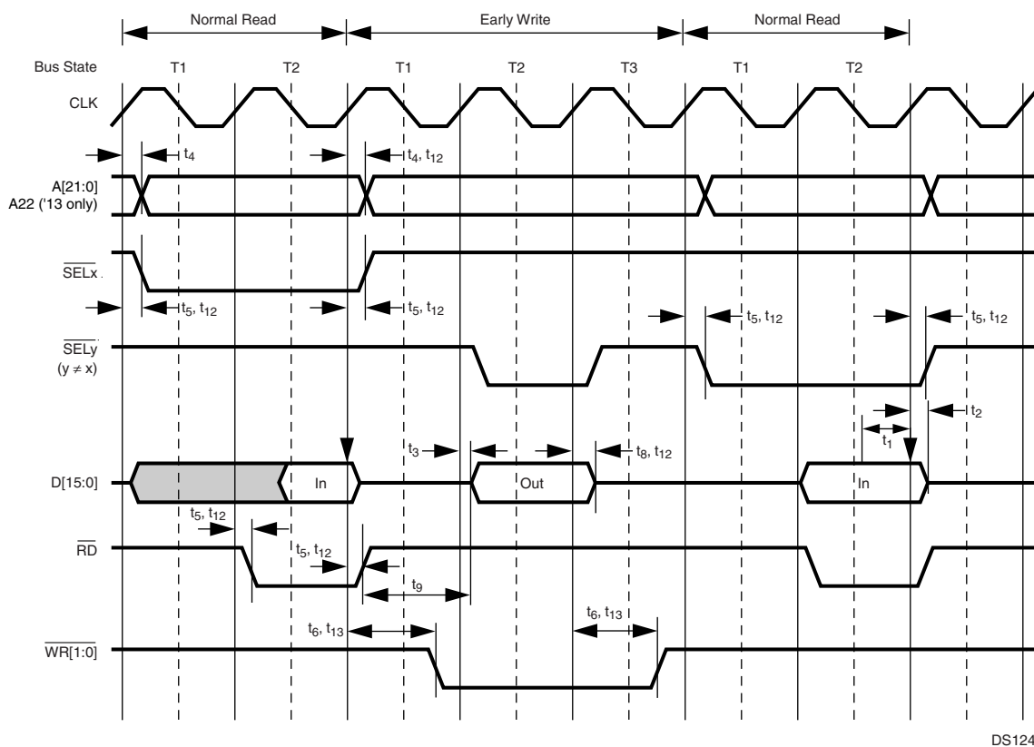
Figure 77. Early Write Between Normal Read Cycles (No Wait States)
