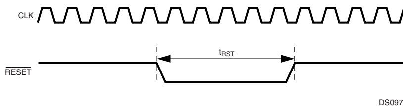
Figure 58. Non-Power-On Reset
