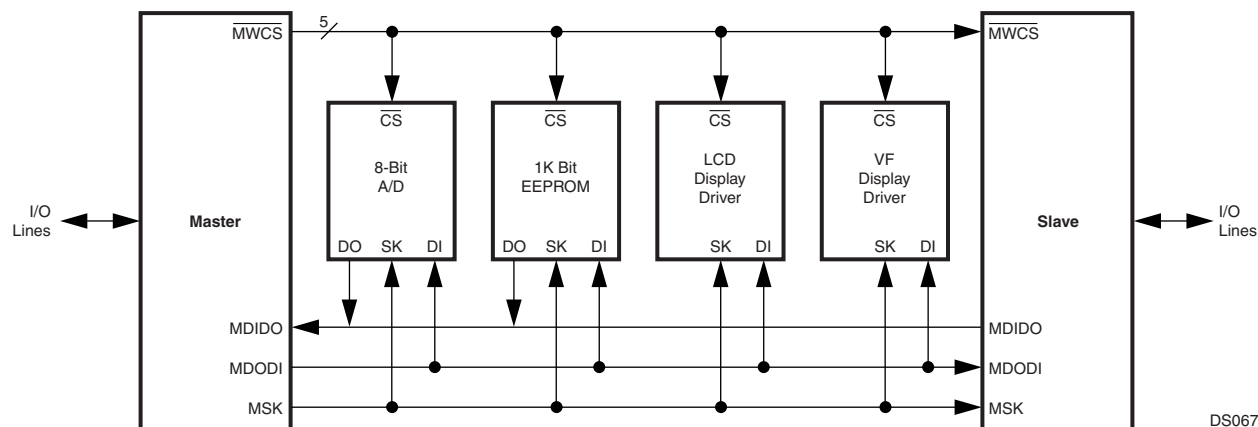
Figure 31. Microwire Interface
