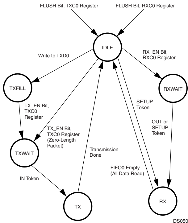
Figure 10. Endpoint 0 Operation
