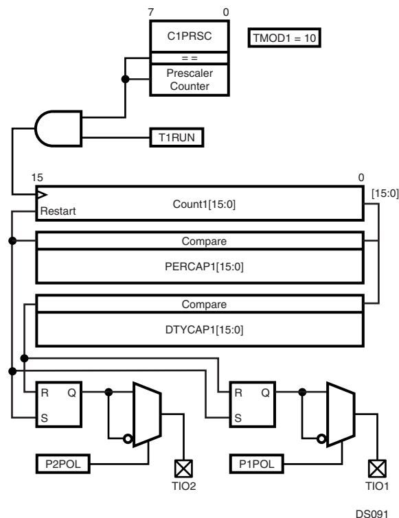
Figure 53. VTU 16-bit PWM Mode
