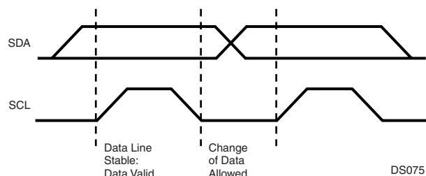
Figure 39. Bit Transfer
