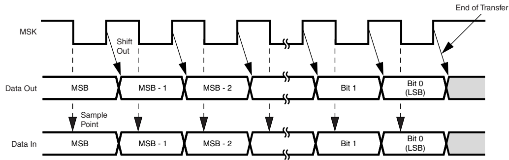
Figure 36. Alternate Mode (SCIDL = 1)
