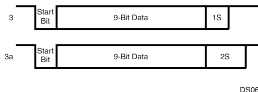
Figure 29. 9-bit Data Frame Options
