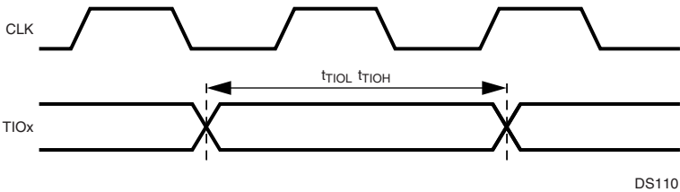
Figure 76. Versatile Timing Unit Input Timing
