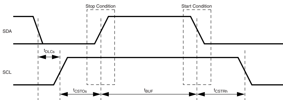
Figure 71. ACB Signals (SDA and SCL) Timing
