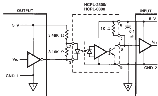
Figure 14. Series Drive from Open Collector TTL/LSTTL
