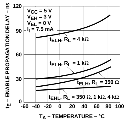
Figure 11. Typical Enable Propagation Delay vs. Temperature.
