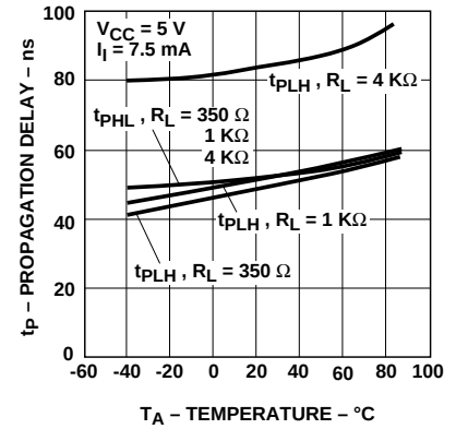
Figure 7. Typical Propagation Delay vs. Temperature.
