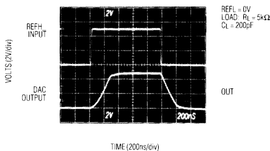
MAX529 FULL-BUFFERED STEP RESPONSE
