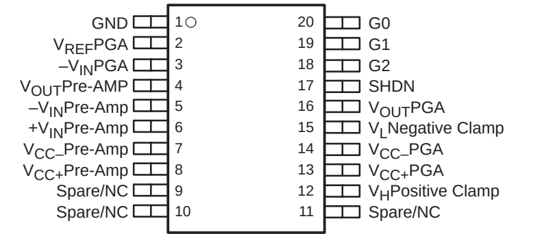
THS7001 PWP PACKAGE (TOP VIEW)
