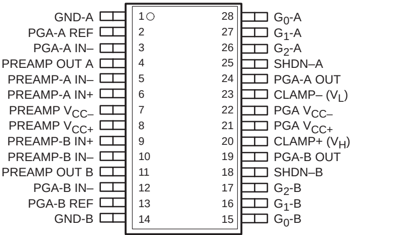
THS7002 PWP PACKAGE (TOP VIEW)
