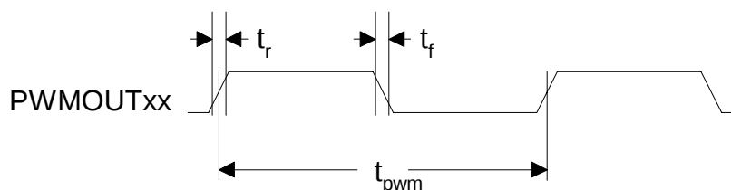
Figure 4. PWMOUTxx Timings
