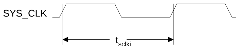
Figure 3. SYS_CLK Timings
