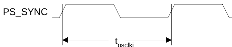
Figure 5. PS_SYNC Timings
