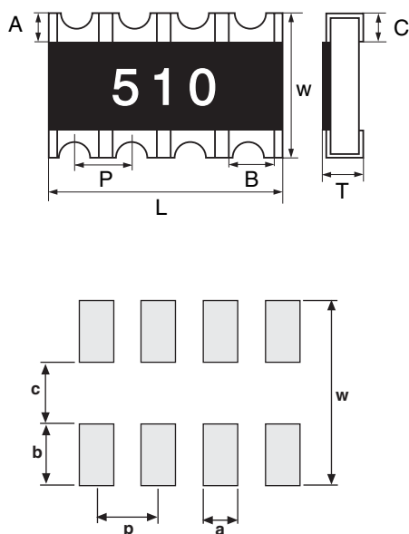
4-Resistor Device
