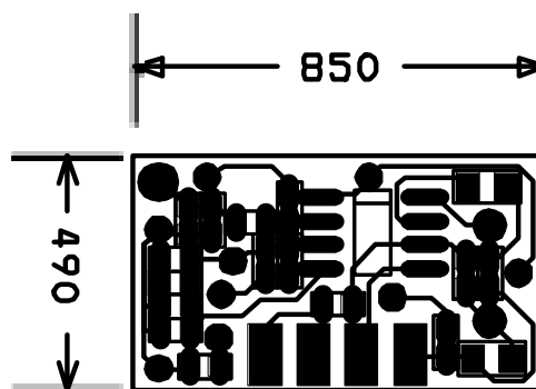
PCB Component Side Layout
