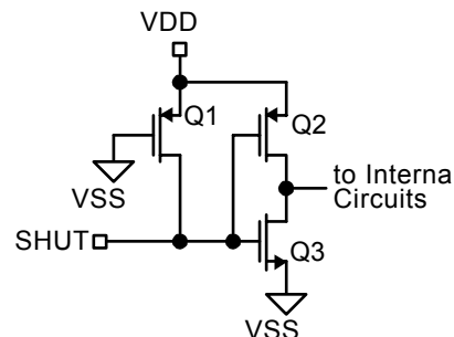
Figure 6. SHUT Pin
