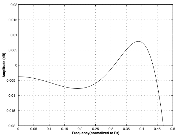
Figure 48. Single Speed (fast) Passband Ripple
