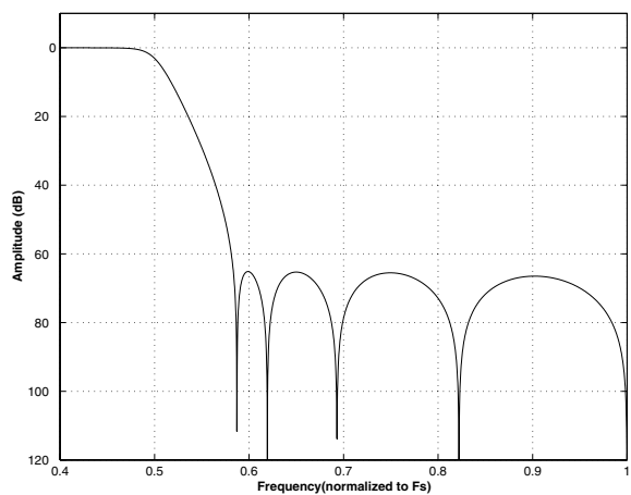
Figure 49. Single Speed (slow) Stopband Rejection
