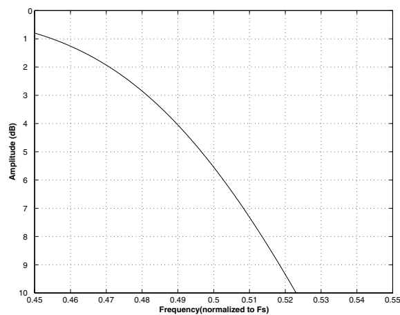
Figure 67. Quad Speed (slow) Transition Band (detail)
