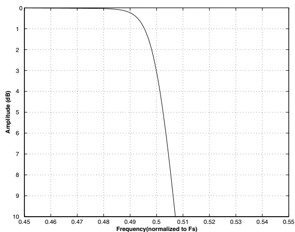
Figure 47. Single Speed (fast) Transition Band (detail)
