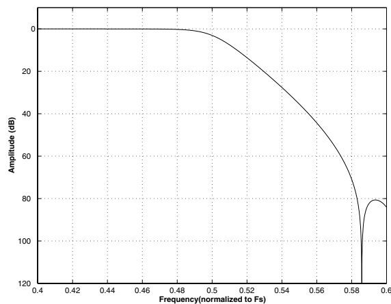
Figure 54. Double Speed (fast) Transition Band
