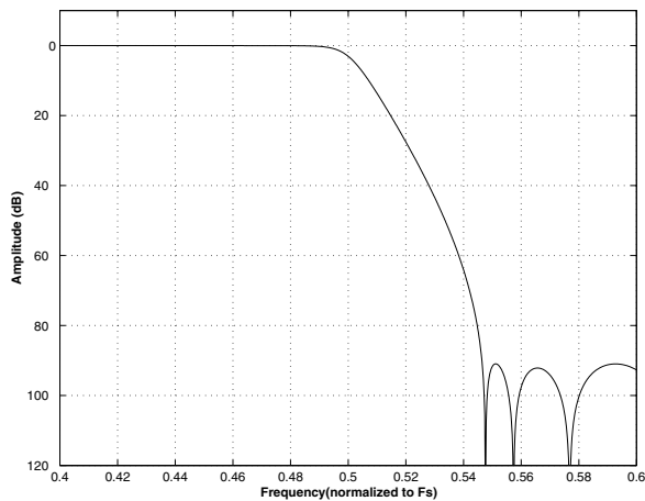
Figure 46. Single Speed (fast) Transition Band
