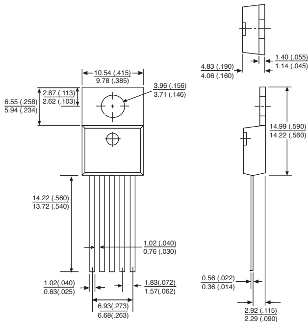
5 Lead TO-220 (TVA) Vertical
