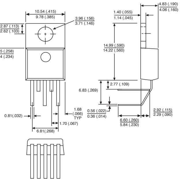
5 Lead TO-220 (THA) Horizontal
