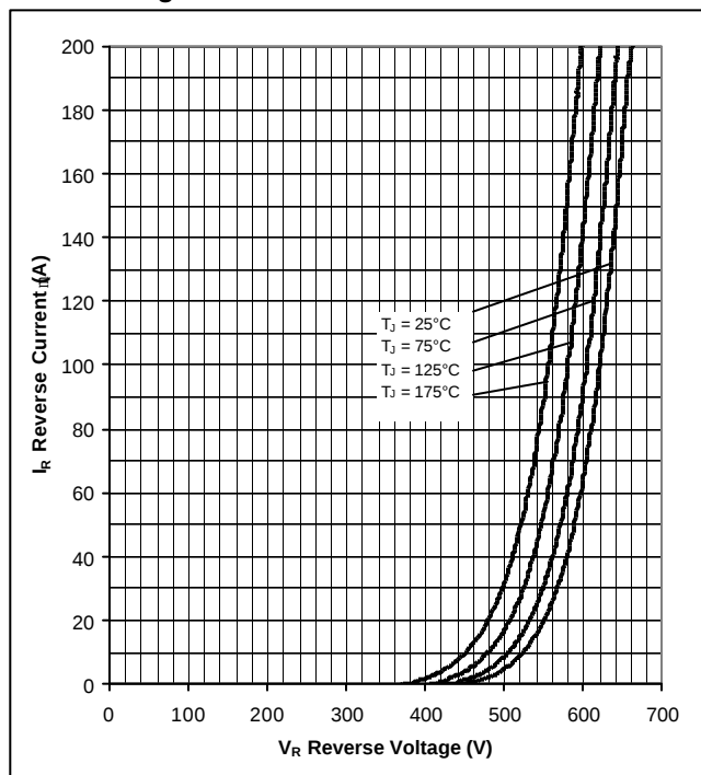
Figure 2. Reverse Characteristics
