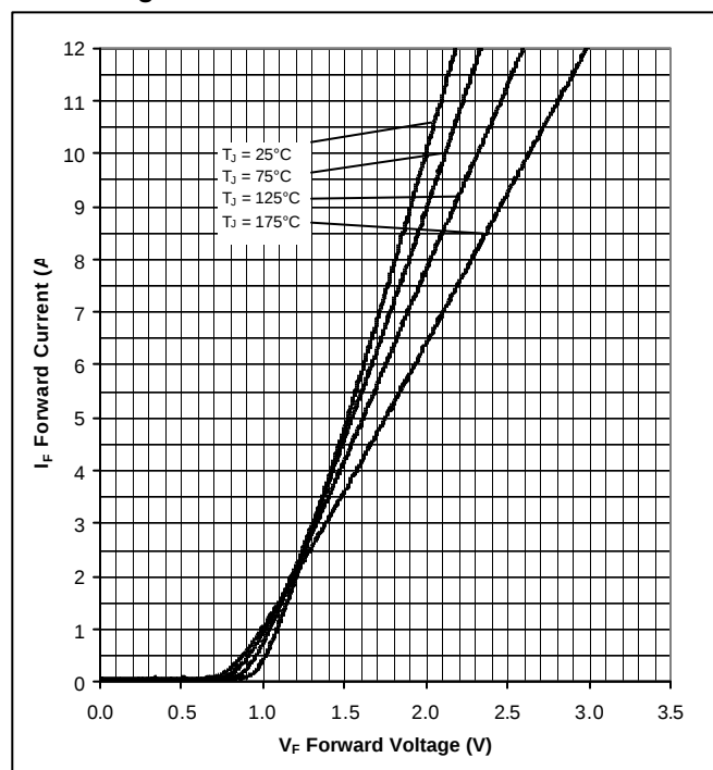
Figure 1. Forward Characteristics
