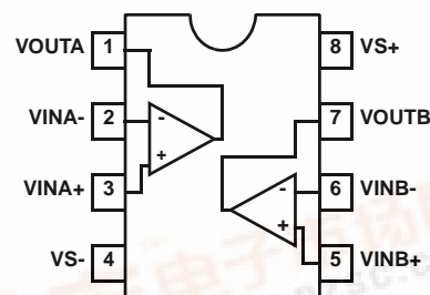
EL2228 (8-PIN SO, MSOP) TOP VIEW
