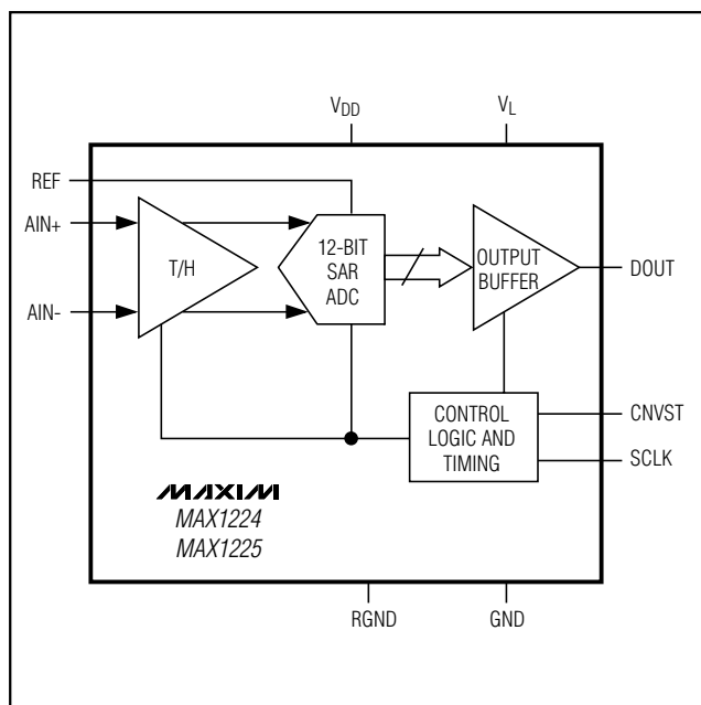
Figure 3. Functional Diagram
