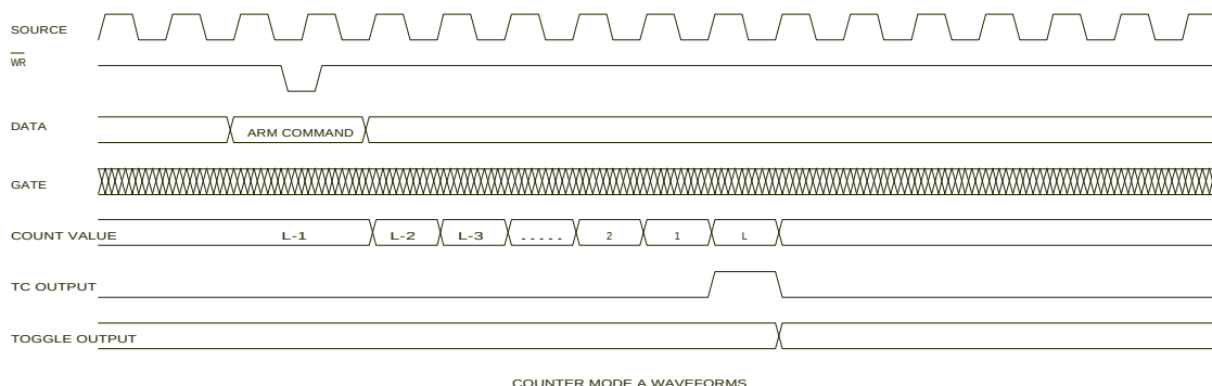
Figure 10 - CTS9513 Counter Mode A Representative Waveforms
