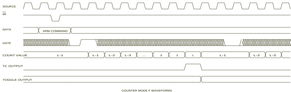
Figure 15 - CTS9513 Counter Mode F Representative Waveforms
