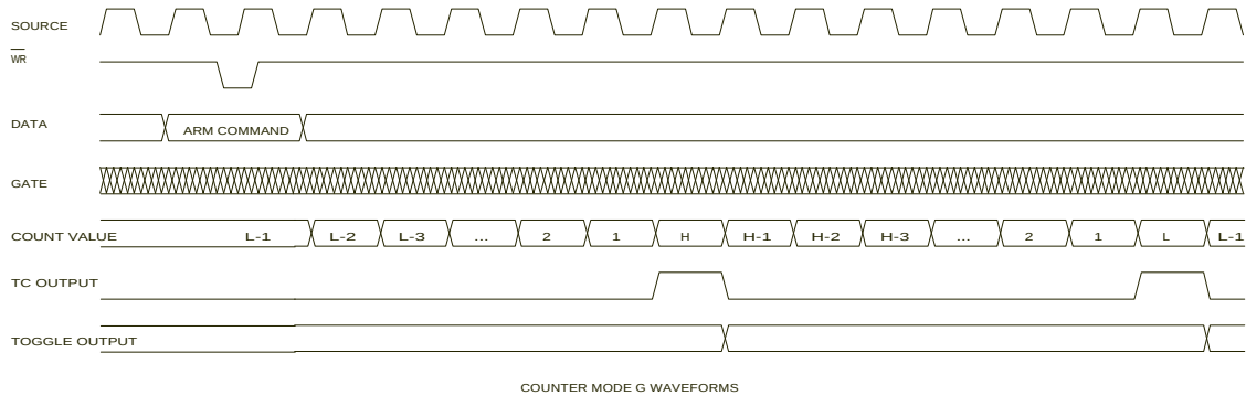
Figure 16 - CTS9513 Counter Mode G Representative Waveforms
