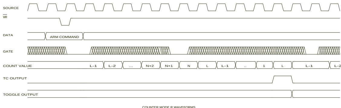
Figure 25 - CTS9513 Counter Mode R Representative Waveforms
