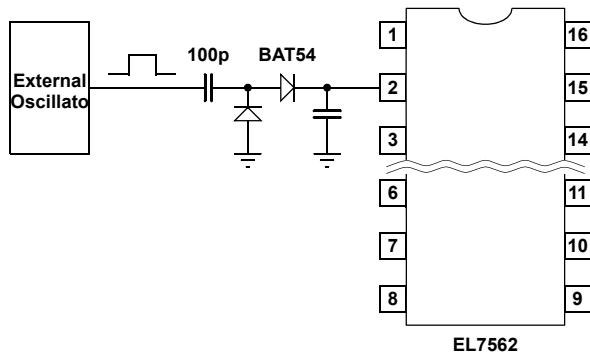
FIGURE 1. Oscillator Synchronization
