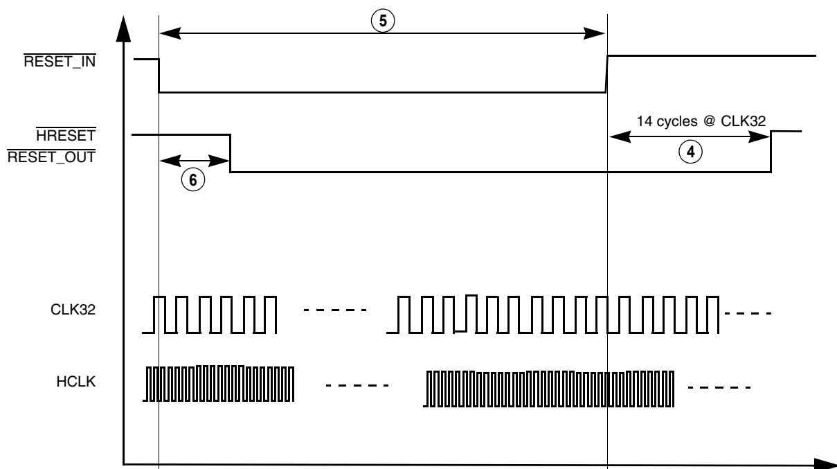
Figure 4. Timing Relationship with RESET_IN
