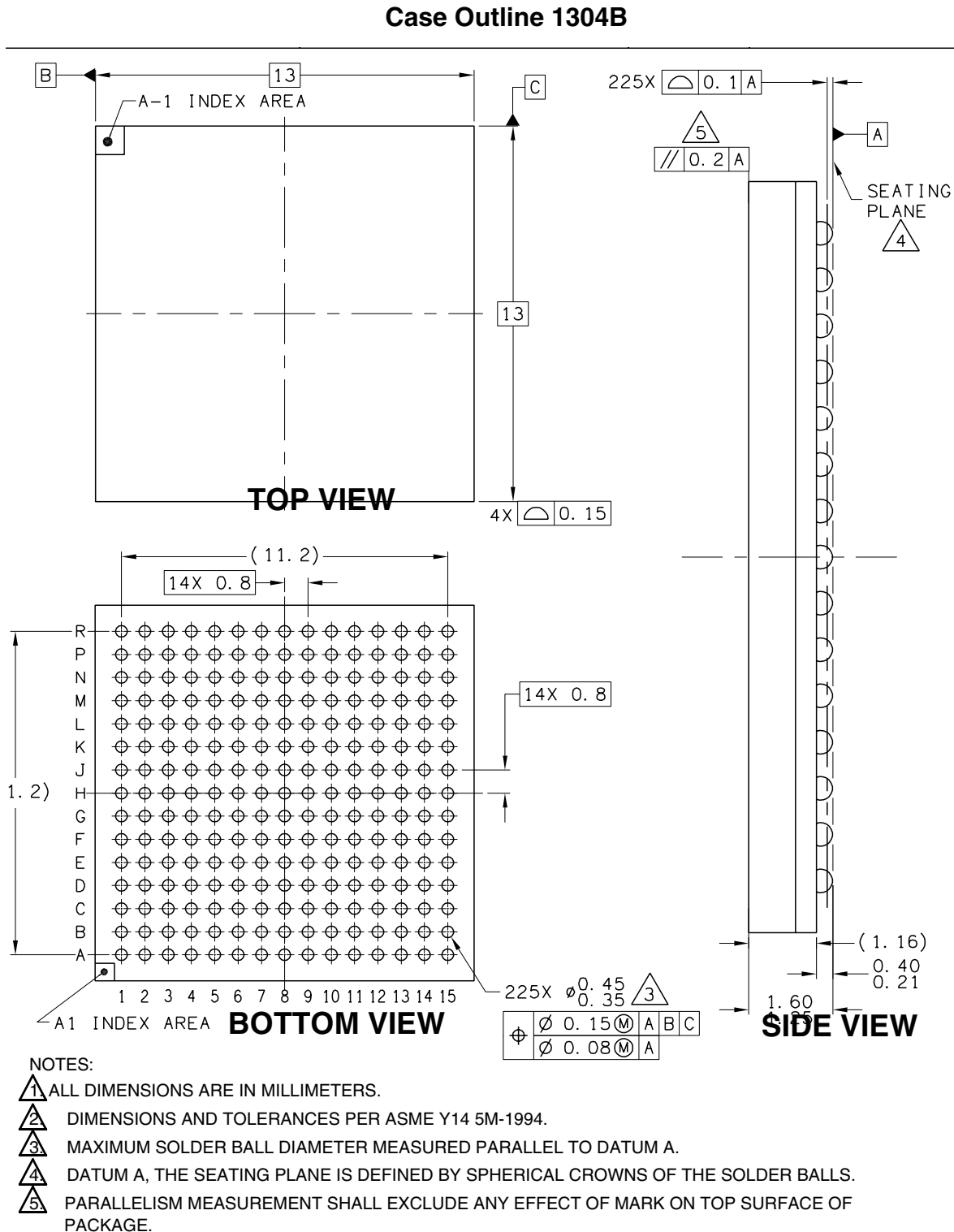
Figure 64. MC9328MXL 225 PBGA Mechanical Drawing
