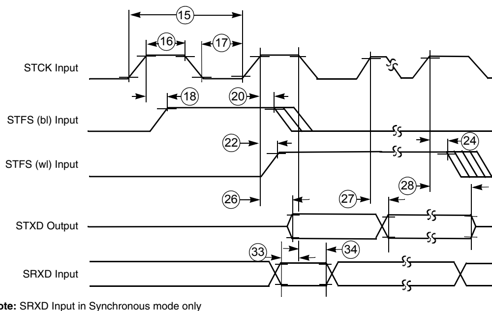
Figure 57. SSI Transmitter External Clock Timing Diagram
