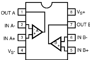
EL2280 (8-PIN SO, PDIP) TOP VIEW
