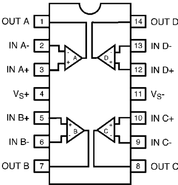
EL2480 (14-PIN SO, PDIP) TOP VIEW
