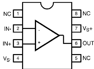
EL2180 (8-PIN SO, PDIP) TOP VIEW
