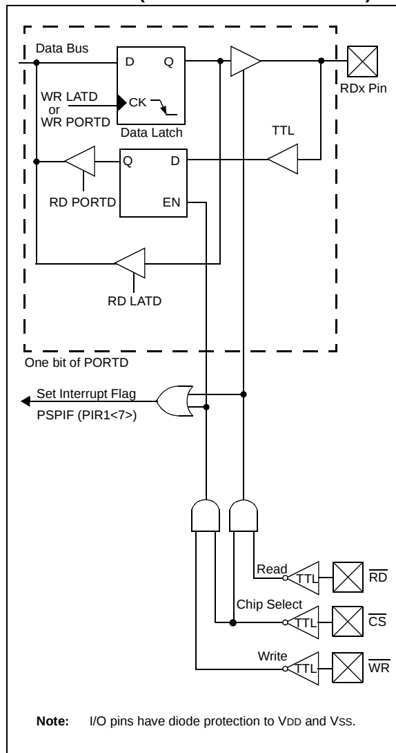
FIGURE 9-1: PORTD AND PORTE BLOCK DIAGRAM (PARALLEL SLAVE PORT)
