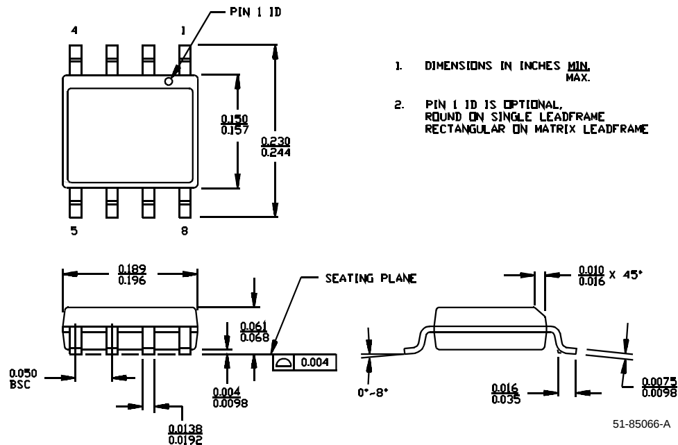
8-pin (150-mil) SOIC S8
