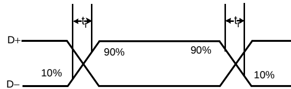
Figure 25-2. USB Data Signal Timing
