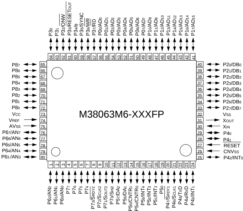
Package type : 80P6N-A 80-pin plastic-molded QFP
