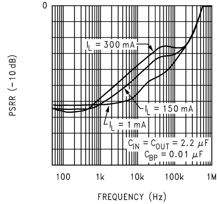
Ripple Rejection ( V_{IN} = V_{OUT} + 1V )
