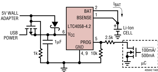
USB/Wall Adapter Power Li-Ion Charger
