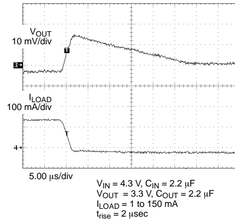
Load Transient Response-2
