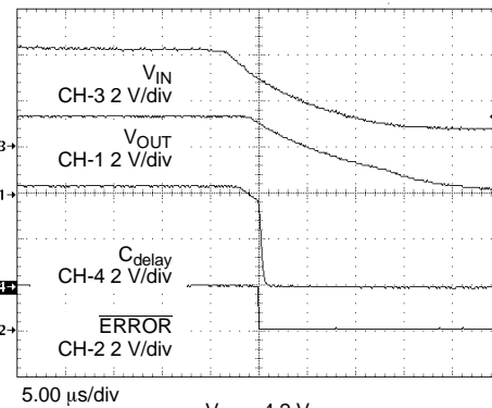
Turn-Off Sequence
