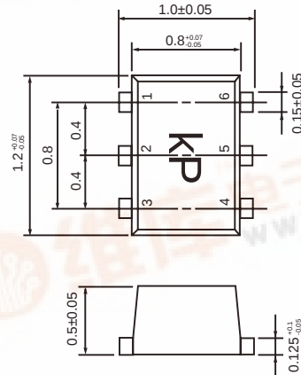
Package Outline TD (TOP VIEW)
