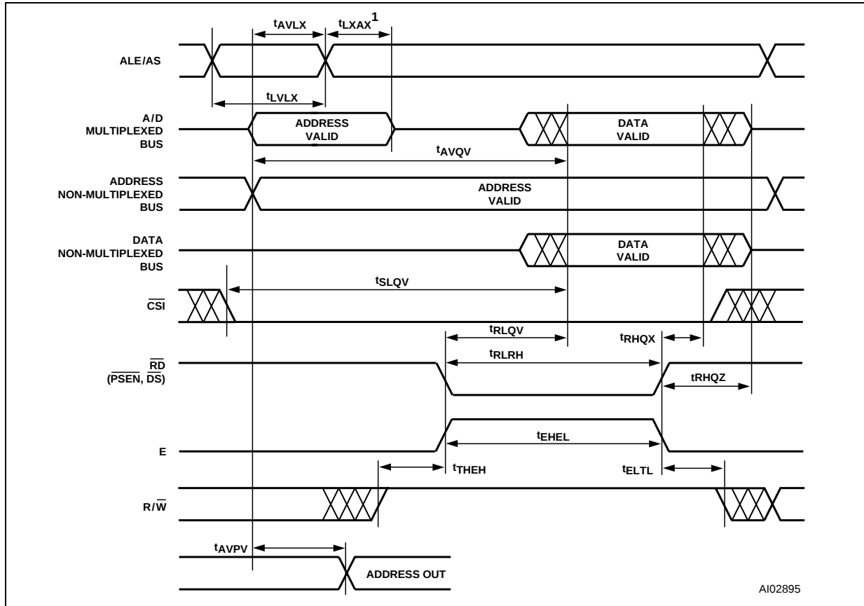
Figure 45. READ Timing
