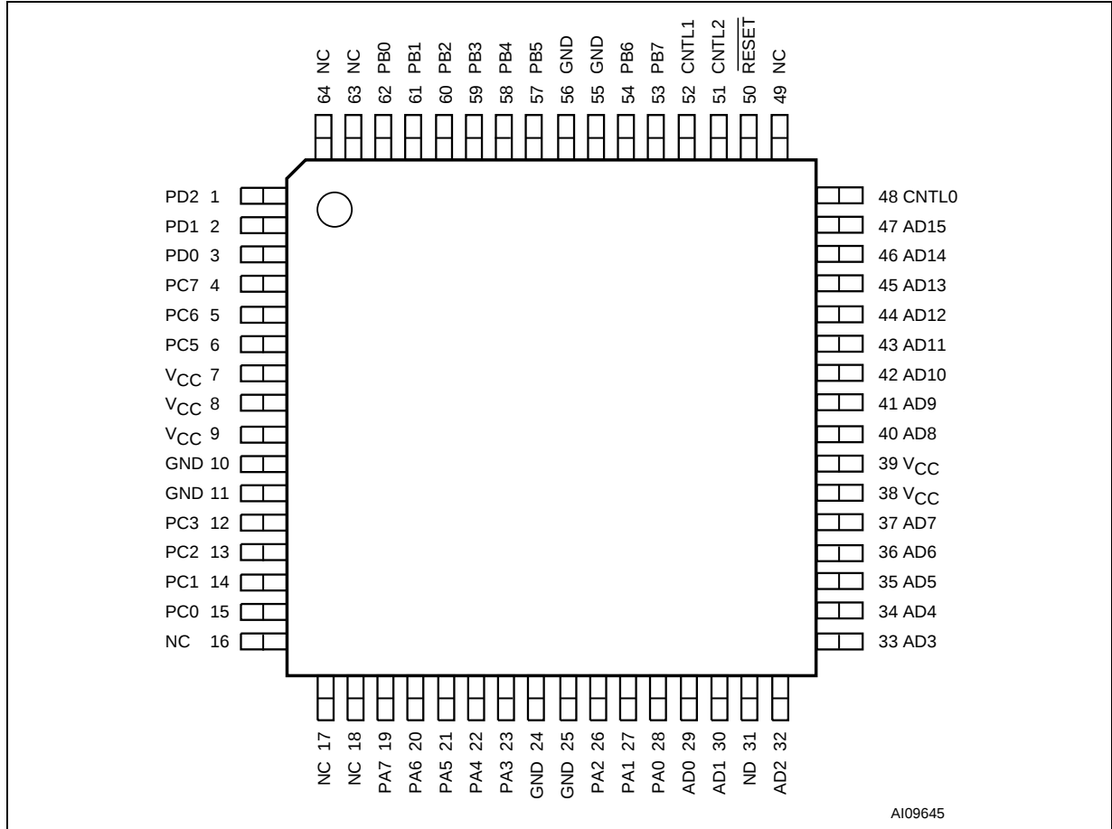
Figure 4. TQFP64 Connections
