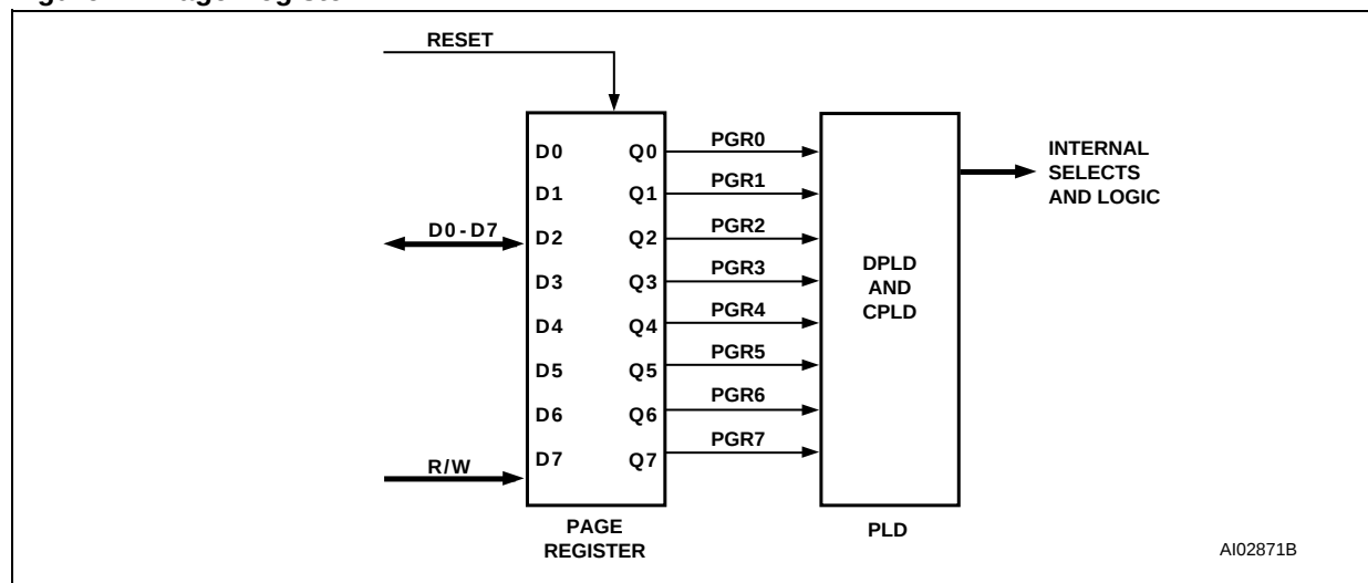
Figure 12. Page Register
