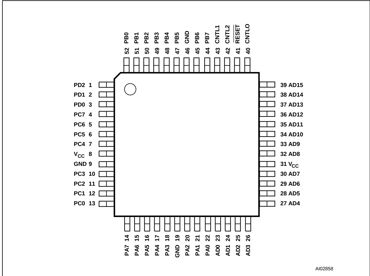
Figure 2. PQFP52 Connections
