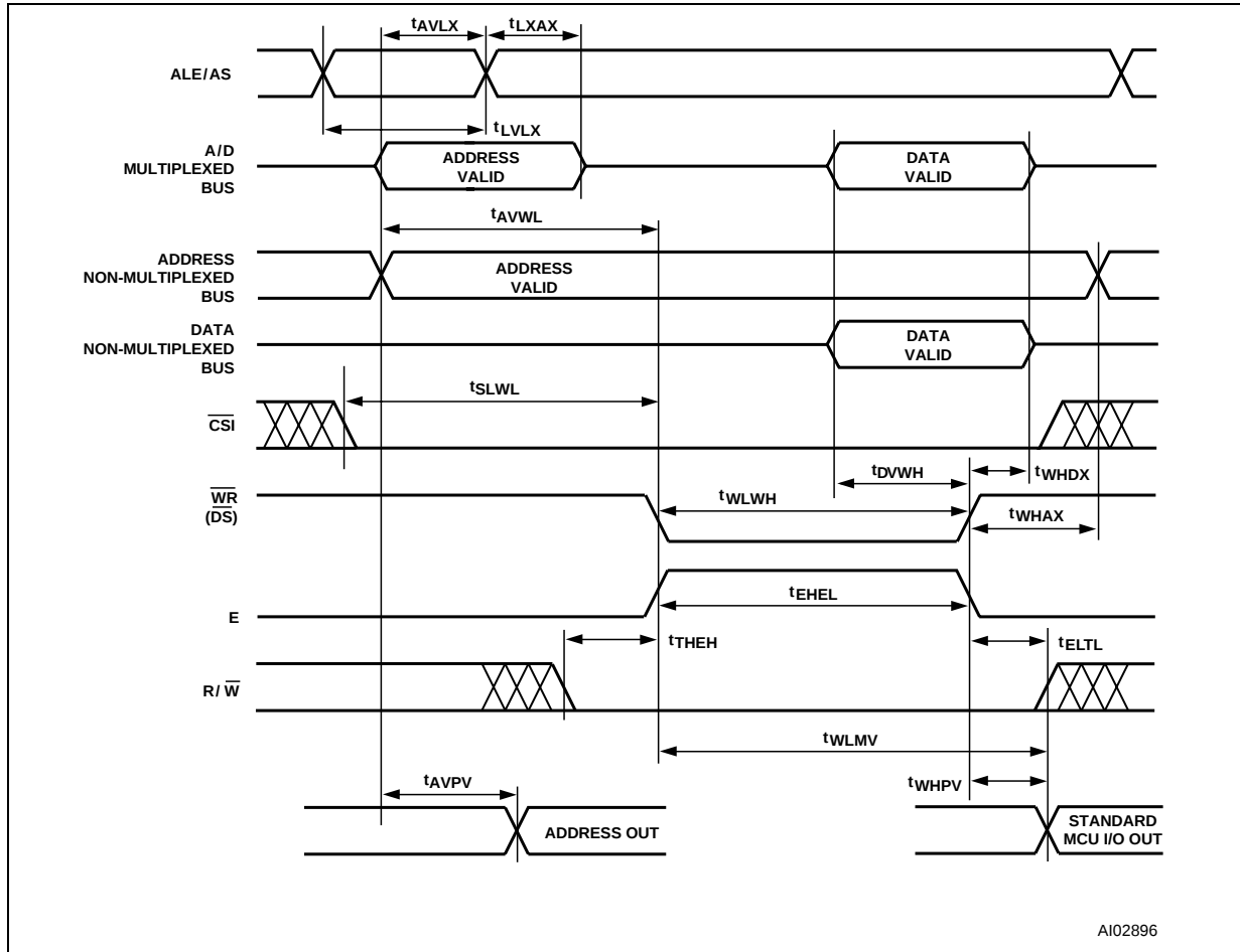
Figure 46. WRITE Timing
