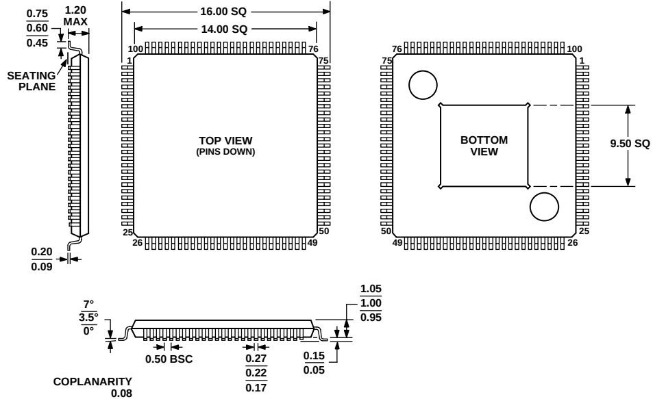
Figure 40. 100-Lead Thin Plastic Quad Flat Package, Exposed Pad [TQFP/EP] (SV-100) Dimensions shown in millimeters
