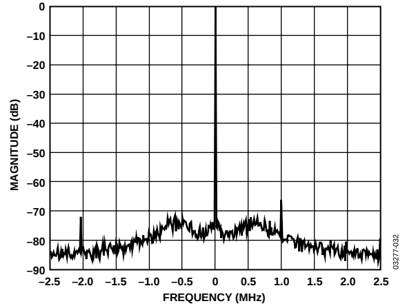
Figure 13. Single Sideband @ 65 MHz, f_c = 66 MHz, f = 1 MHz, R_{SET} = 10 k \Omega ( I_{OUT} = 4 mA), RBW = 500 Hz
