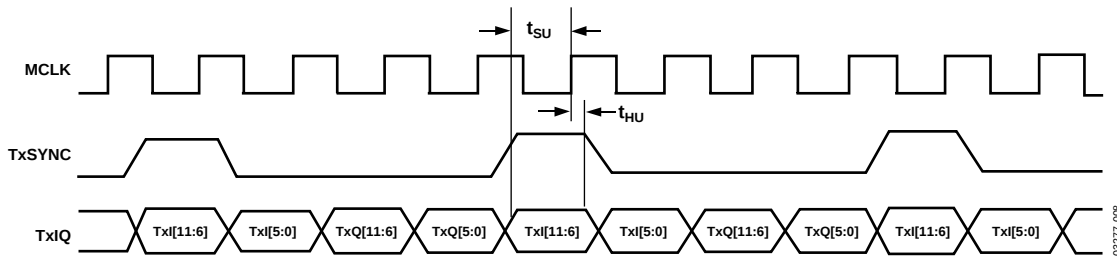
Figure 24. Tx Timing Diagram
