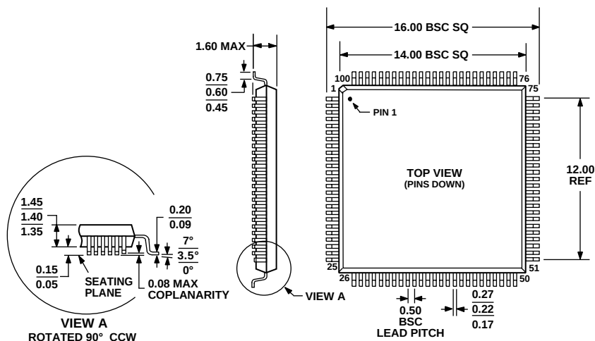
Figure 46. 100-Lead Low Profile Quad Flat Package [LQFP] (ST-100)
