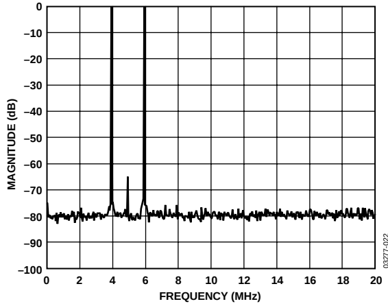
Figure 3. Dual-Sideband Spectral Plot, f_c = 5 MHz, f = 1 MHz, R_{SET} = 10 k \Omega ( I_{OUT} = 4 mA), RBW = 1 kHz
