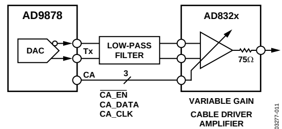
Figure 27. Cable Amplifier Connection
