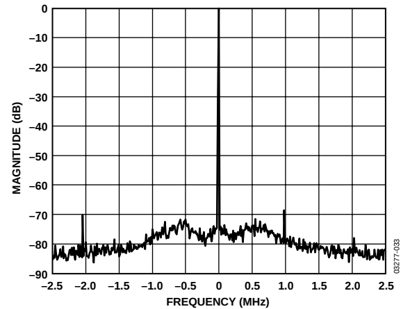
Figure 14. Single Sideband @ 65 MHz, f_c = 66 MHz, f = 1 MHz, R_{SET} = 4 k \Omega ( I_{OUT} = 10 mA), RBW = 500 Hz
