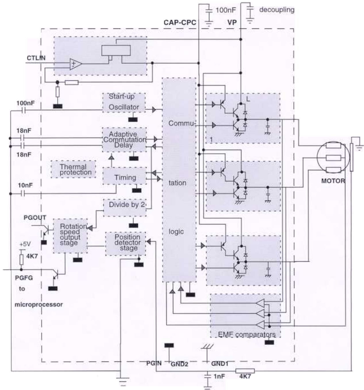
Fig.5 Typical application of the TDA5240T.
