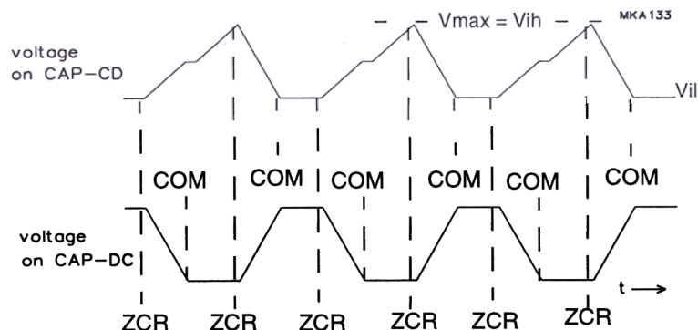
Fig.7 CAP-CDM and CAP-CDS voltage waveforms in normal running mode. (ZCR=ZERO-CROSSING ; COM=COMMUTATION)
