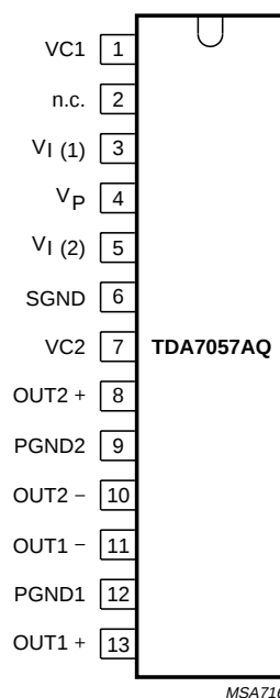
Fig.2 Pin configuration.
