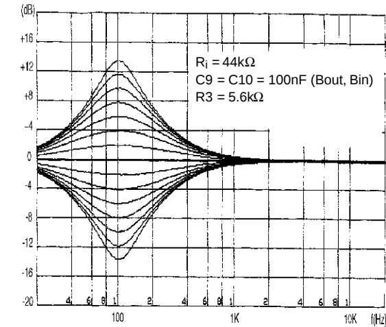
Figure 10: Bass response
