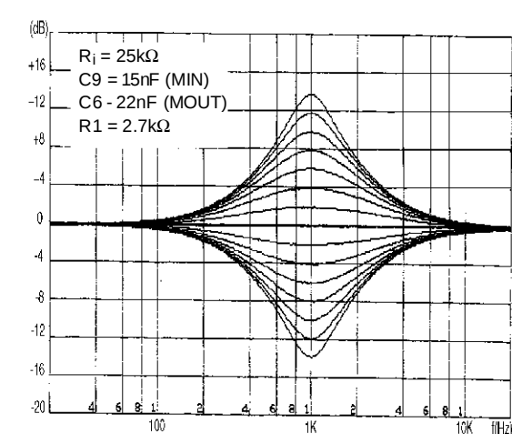
Figure 11: Middle response
