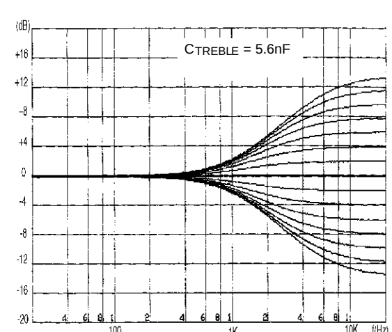
Figure 12: Treble response
