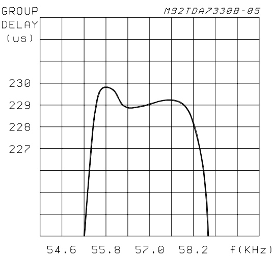
Figure 6: Group Delay vs. Frequency
