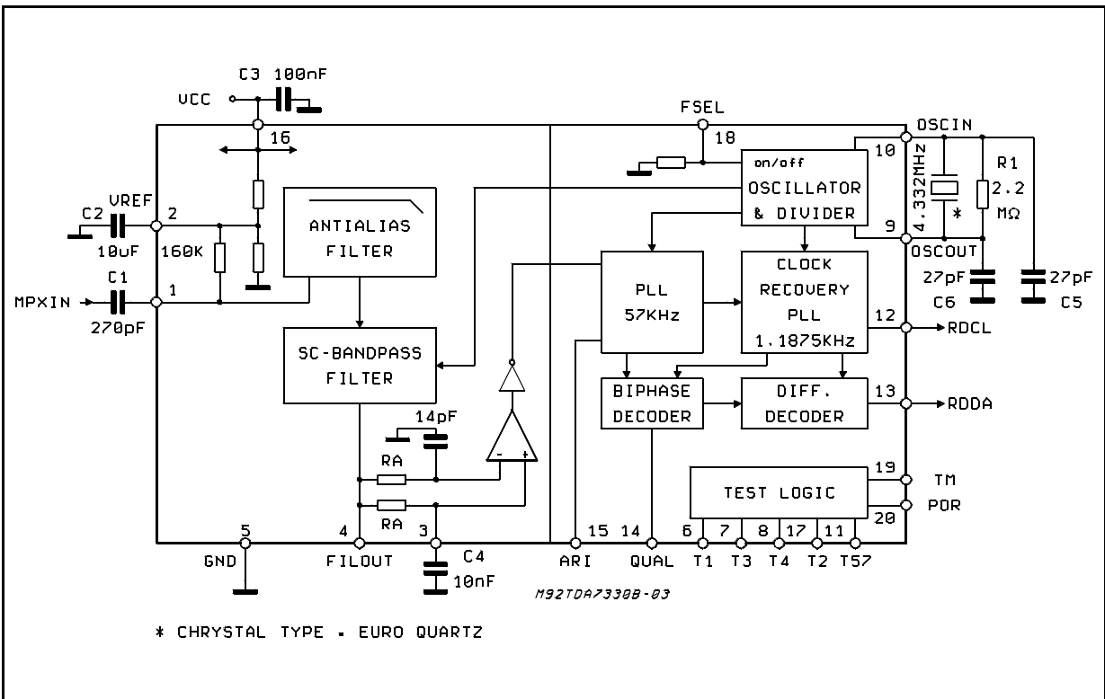
Figure 3: Test Circuit
