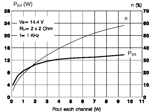
Figure 11: Total Power Dissipation and Efficiency
