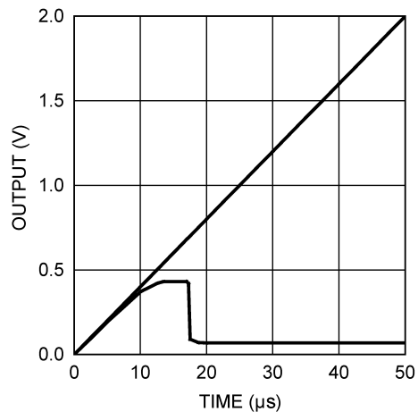
Power-On Reset
