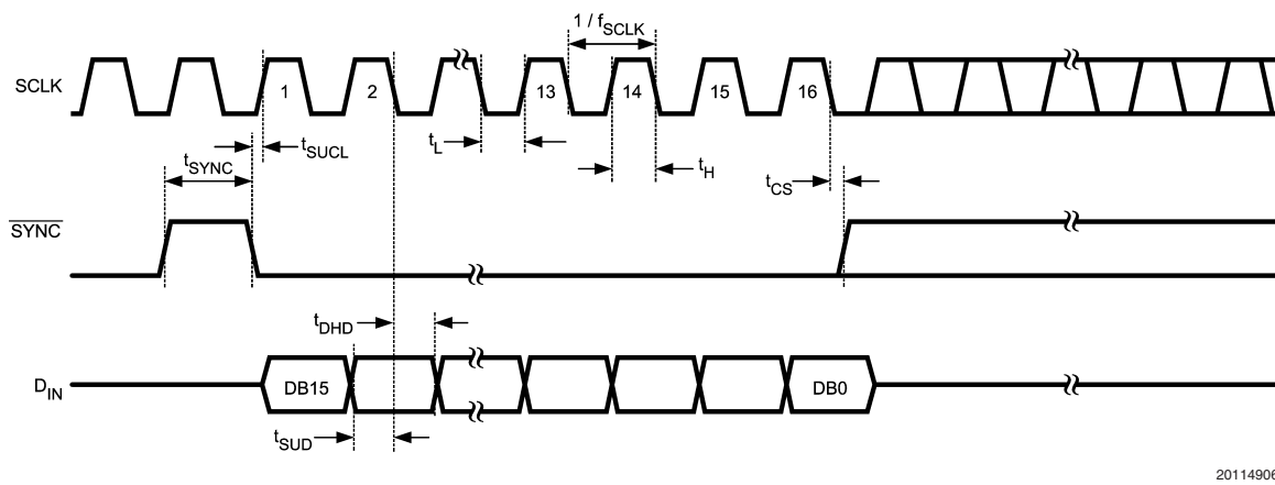
FIGURE 2. DAC121S101 Timing
