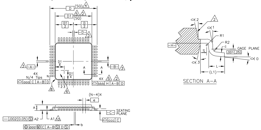
Package Number 355 - 48-Lead TGFP, 1.0 mm Thick, 7.0 x 7.0 mm Body
