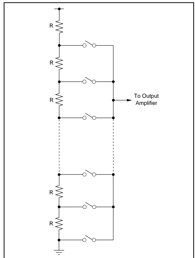
FIGURE 2. Resistor String.
