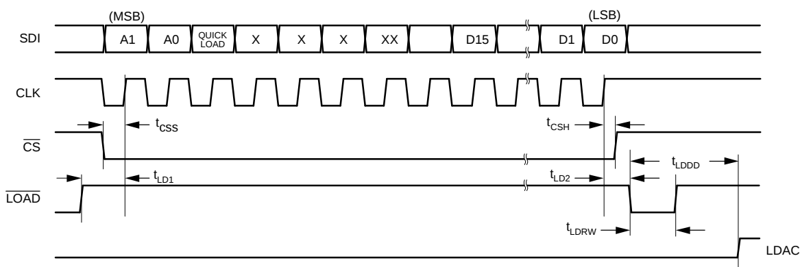
Figure 62. Serial Interface Timing
