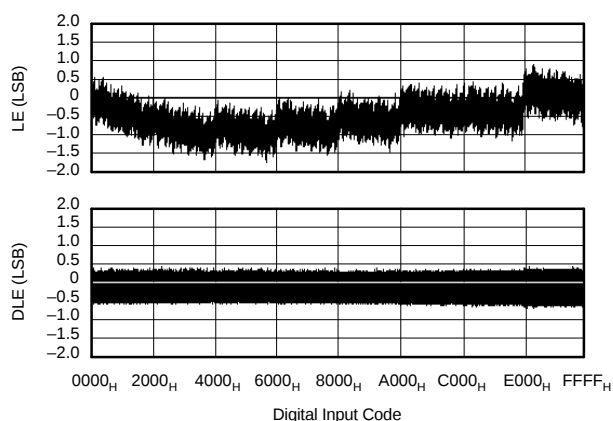
Figure 54. Integral Linearity and Differential Linearity Error Curves for Figure 53
