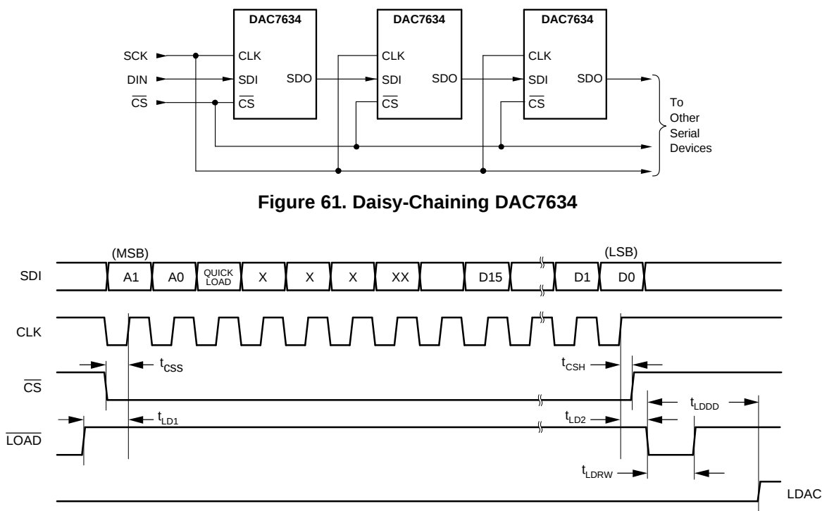
Figure 62. Serial Interface Timing
