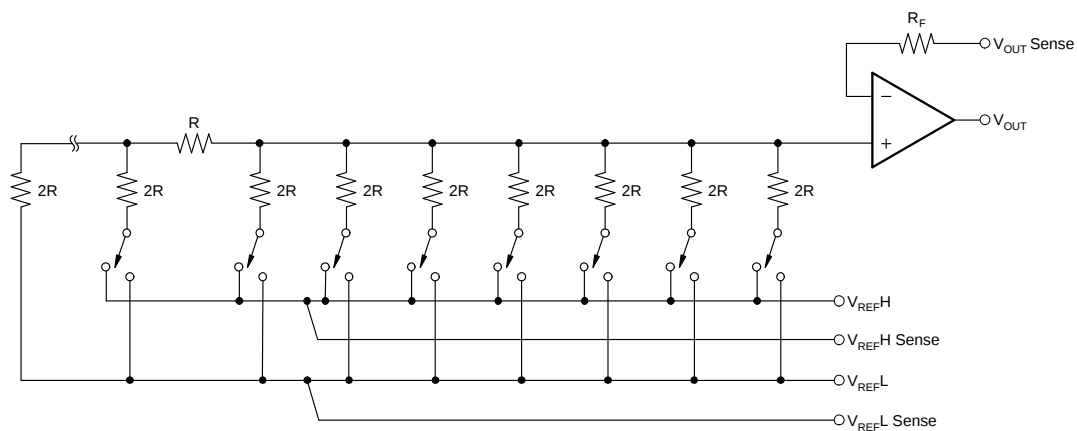
Figure 48. DAC7634 Architecture
