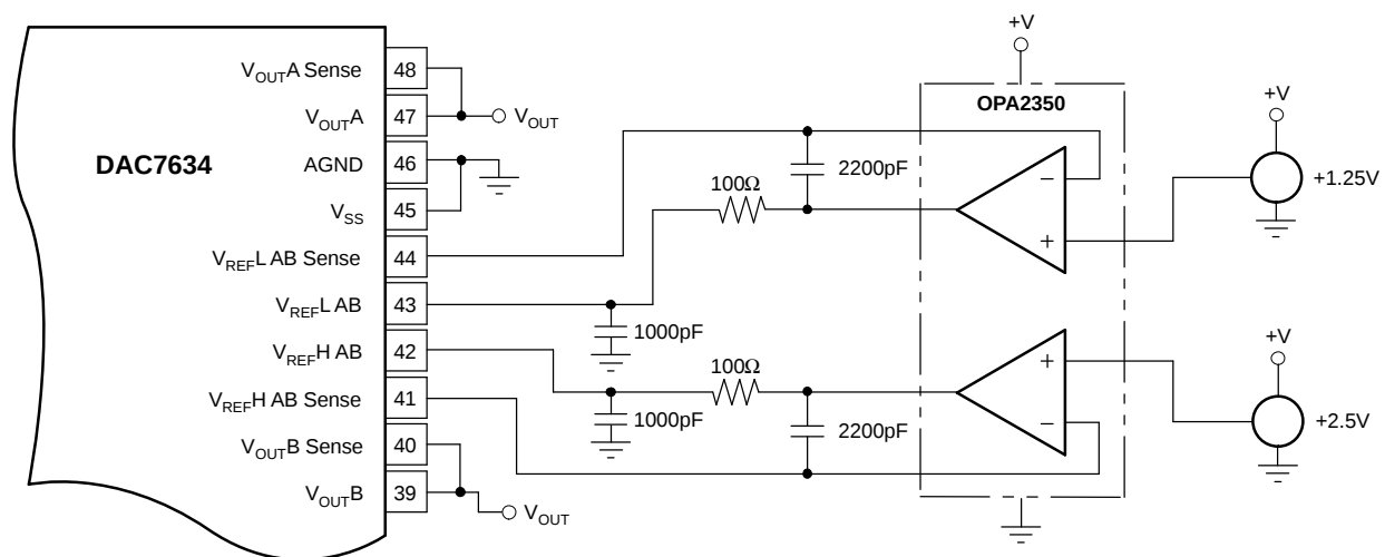
Figure 56. Single-Supply Buffered Reference With V_{REFH} = 2.5 V and V_{REFL} = 1.25 V (1/2 DAC7634)
