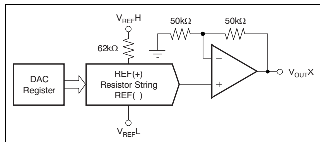
Figure 92. DAC7564 Architecture
