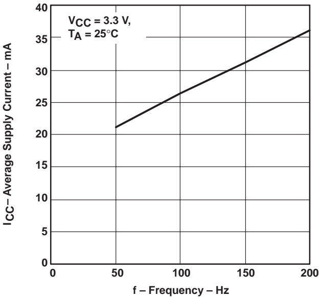
Figure 13. Average Supply Current vs Frequency
