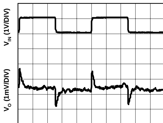
Transient Line Response
